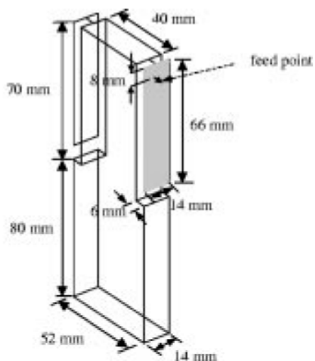
Side-mounted patch
